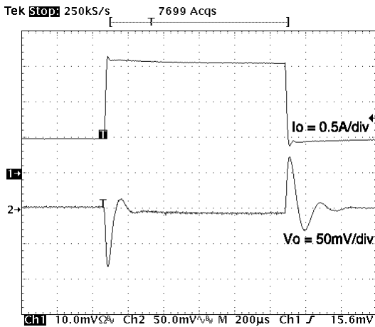
Figure 25. Line transient.
