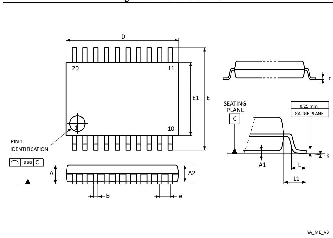
Figure 30.TSSOP20 outline
