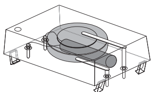
SNAPHAT® battery with crystal
