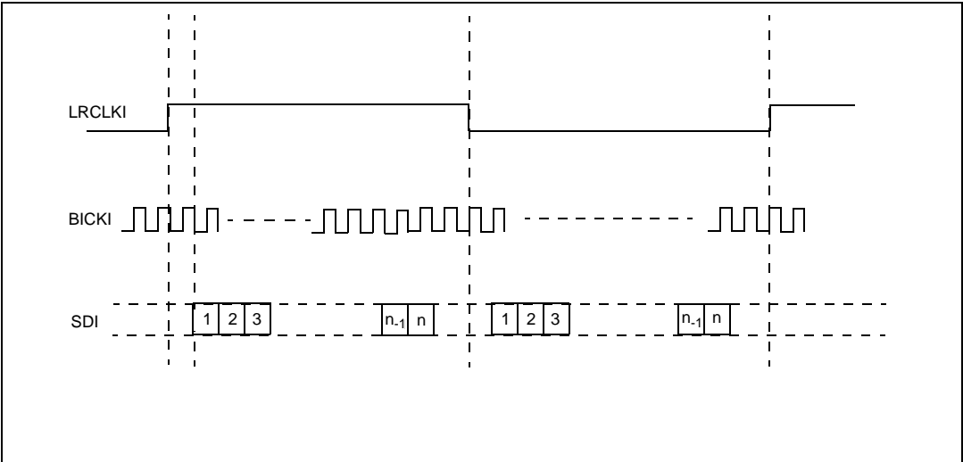
Figure 7. I²S
