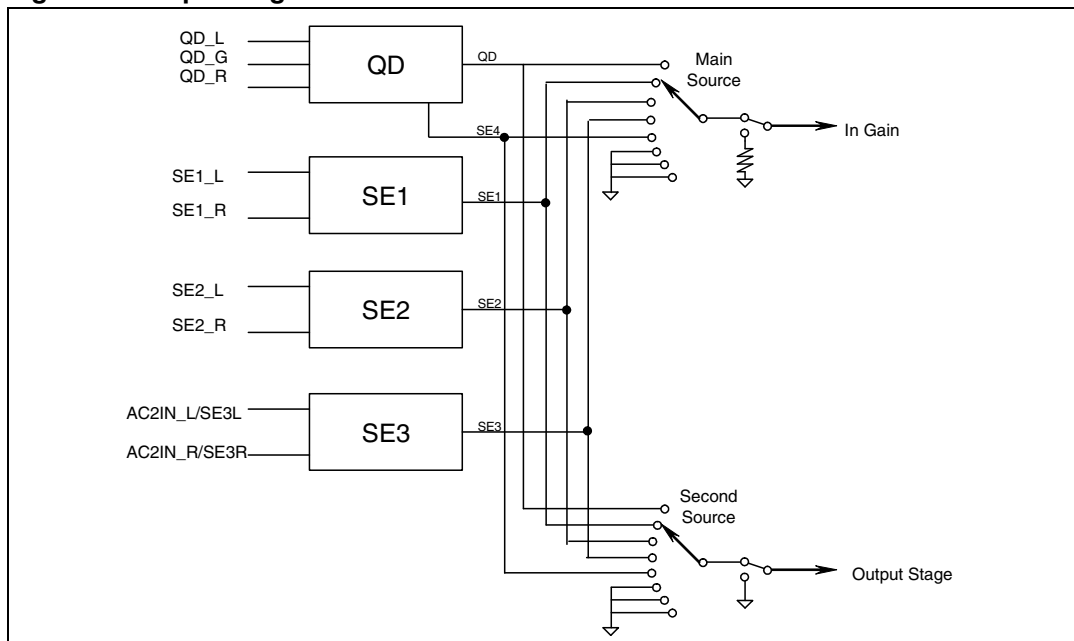
Figure 3. Input stage
