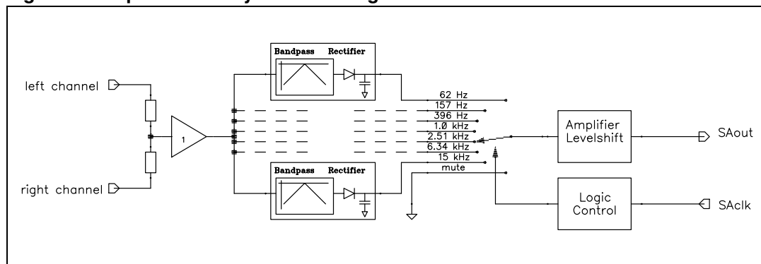
Figure 19. Spectrum analyzer block diagram
