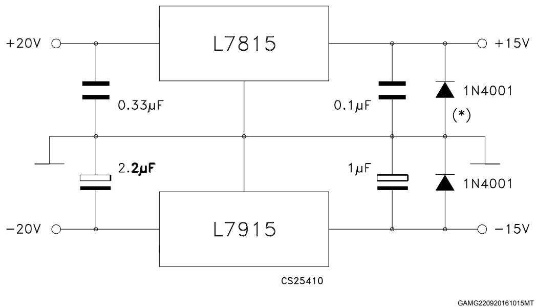
Figure 17. Split power supply ( \pm 15 V - 1 A )
