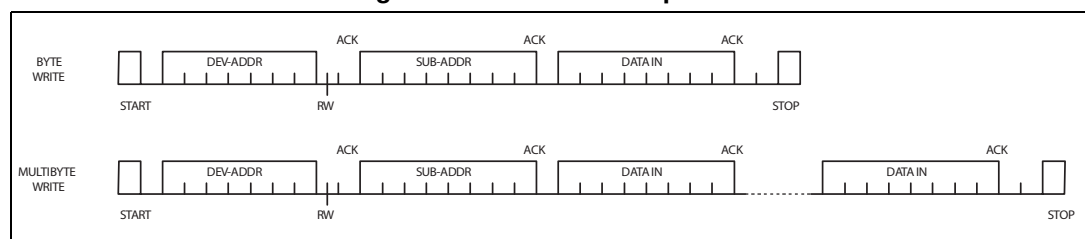
Figure 8. Write-mode sequence
