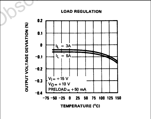
Figure 6. Load regulation
