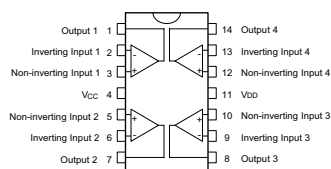
TS464CD-TS464CPT
