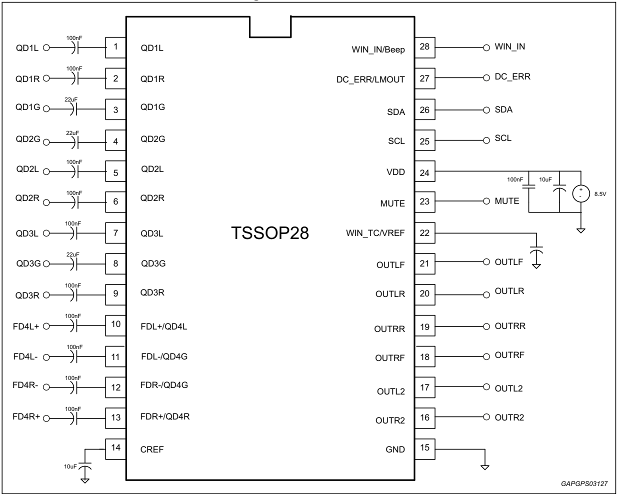
Figure 20. Test circuit
