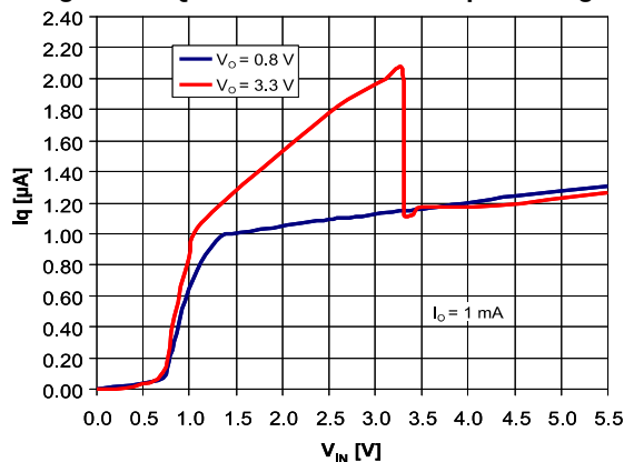
Figure 12: Quiescent current vs input voltage
