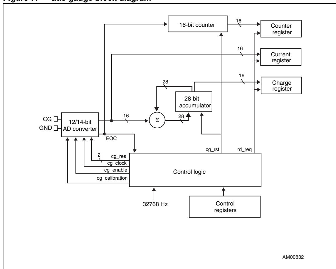
Figure 7. Gas gauge block diagram
