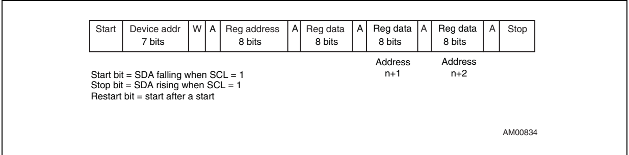
Figure 9. Write operation
