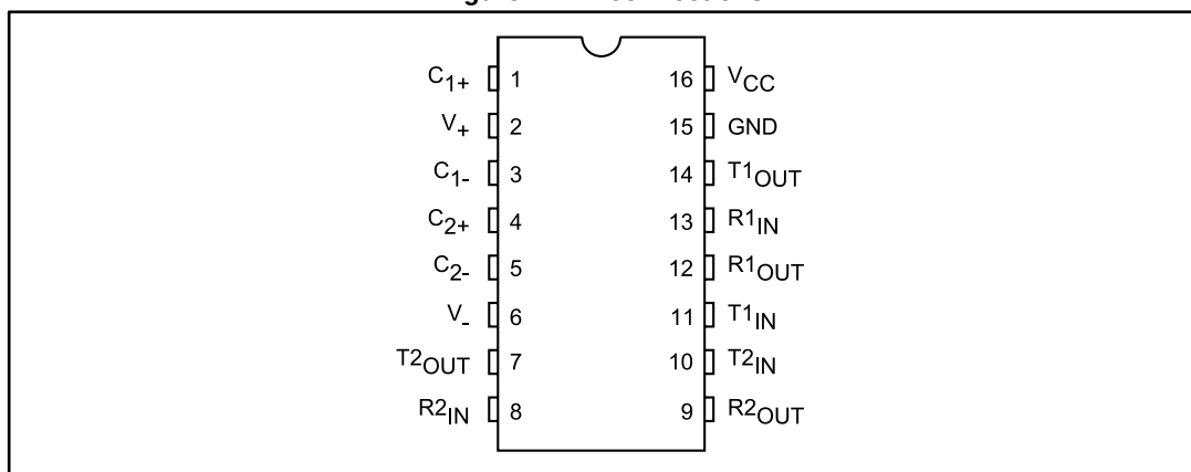
Figure 1: Pin connections
