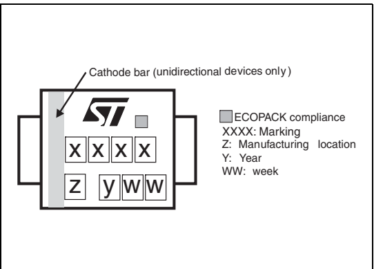
Figure 18. Marking layout (1)
