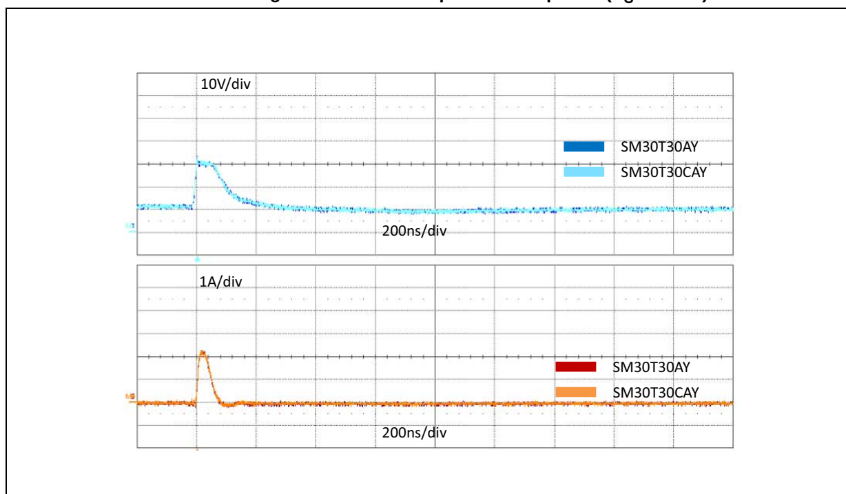
Figure 15. ISO7637-2 pulse 3b response ( V_S = 150\text{ V} )
