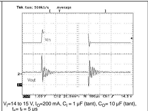
Figure 27. Line transient
