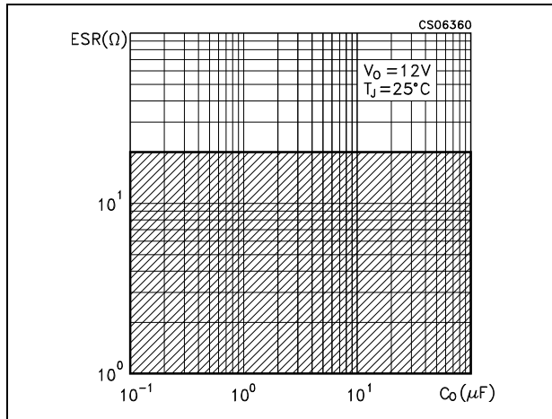
Figure 26. Stability
