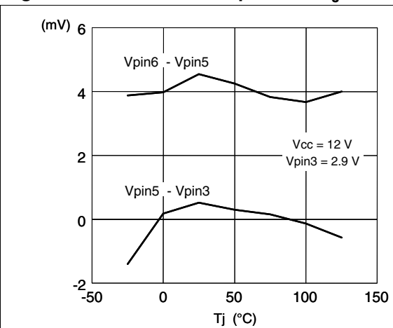
Figure 21. VFF & TBO dropouts vs T_J
