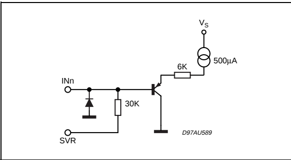
Figure 15. PINS: INL,INR
