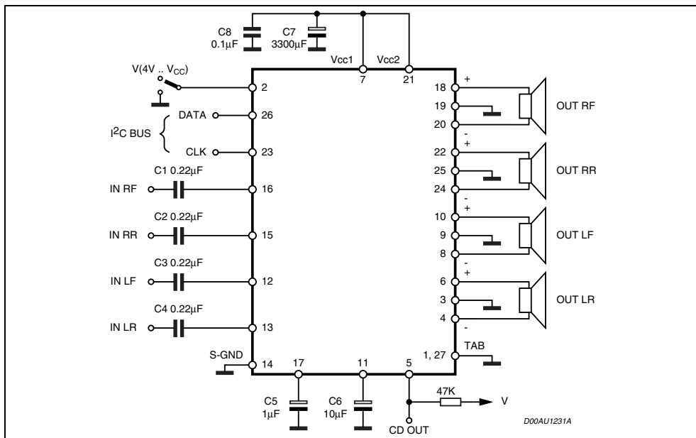
Figure 1. Application Circuit
