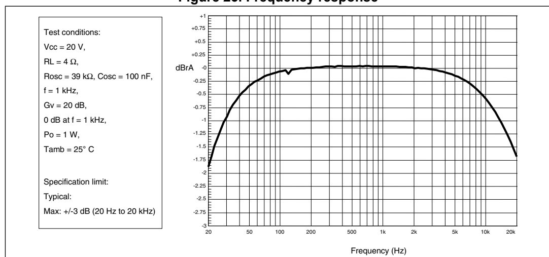
Figure 23. Frequency response
