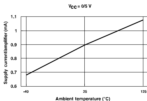
Figure 4: Supply current vs. temperature
