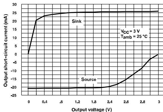
Figure 2: Output short-circuit current vs. output voltage
