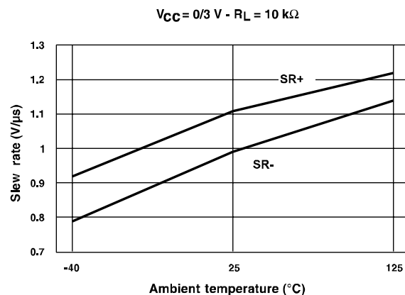
Figure 6: Slew rate vs. temperature
