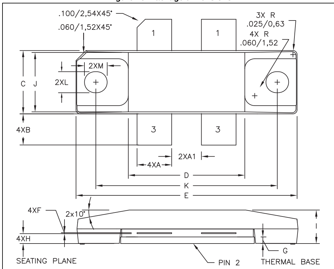
Figure 15. Package dimensions
