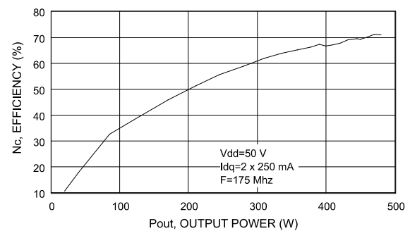
Figure 13: Efficiency vs. output power
