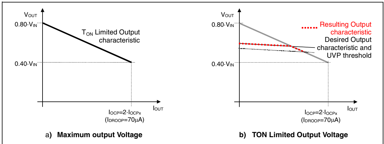
Figure 9. TON Limited Operation
